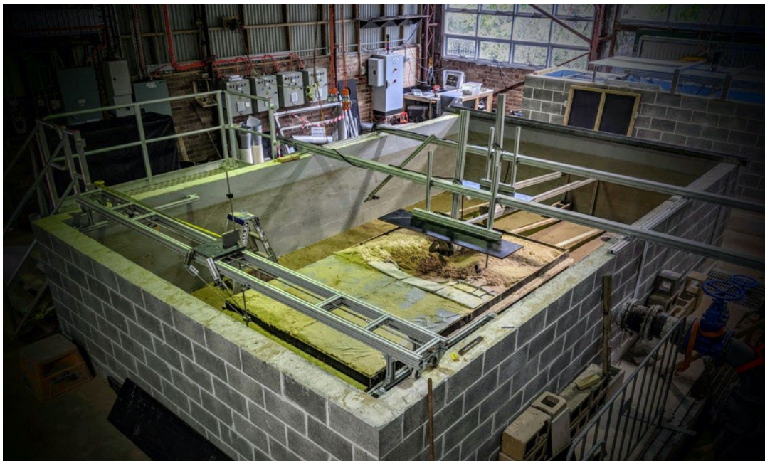
Figure 3 WRL's Prop-Wash Basin
